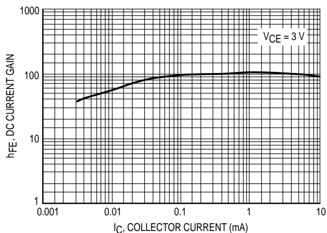
Figure 5. DC Current Gain versus Collector Current
