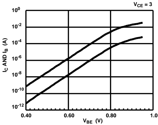
FIGURE 3. GUMMEL PLOT
