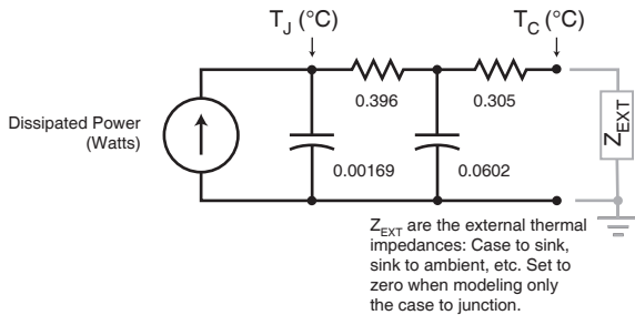
Figure 20, Transient Thermal Impedance Model
