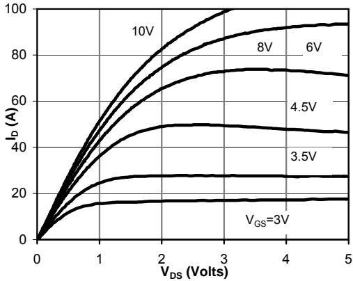
Fig 1: On-Region Characteristics
