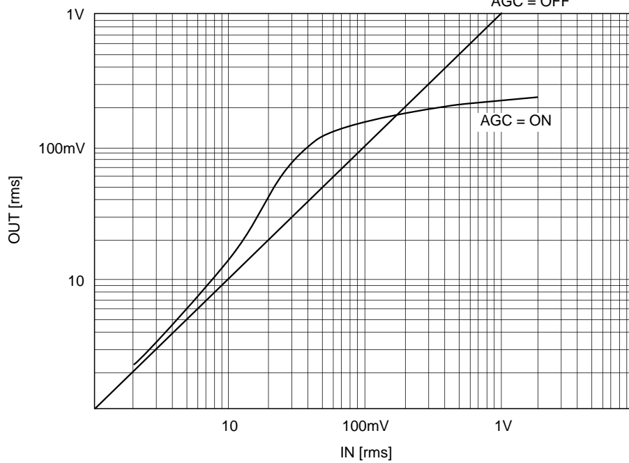
AGC characteristic
