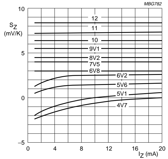
BZV55-B/F/C4V7 to B/F/C12.
