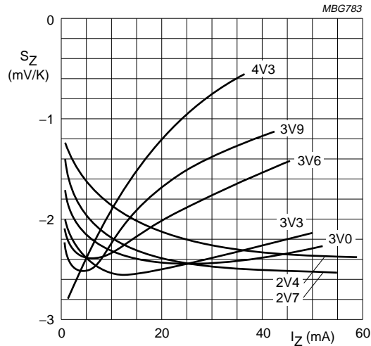
BZV55-B/F/C2V4 to B/F/C4V3.
