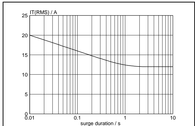
Fig.5. Maximum permissible repetitive rms on-state current I_{T(RMS)} , versus surge duration, for sinusoidal currents, f = 50\text{ Hz} ; T_{hs} \leq 56^\circ\text{C} .
