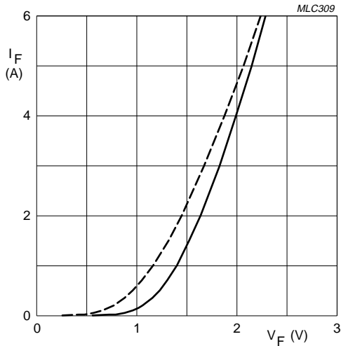
BYD43U and V Dotted line: T_j = 175\text{ °C} . Solid line: T_j = 25\text{ °C} .
