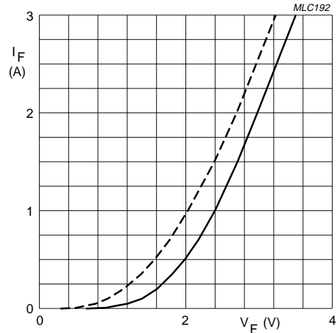
BYD43-16 to 20 Dotted line: T_j = 175\text{ °C} . Solid line: T_j = 25\text{ °C} .
